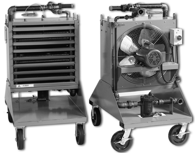
CAQ-202-HS-T12 (380 MBH - 50 psig @ 60°F EAT)
