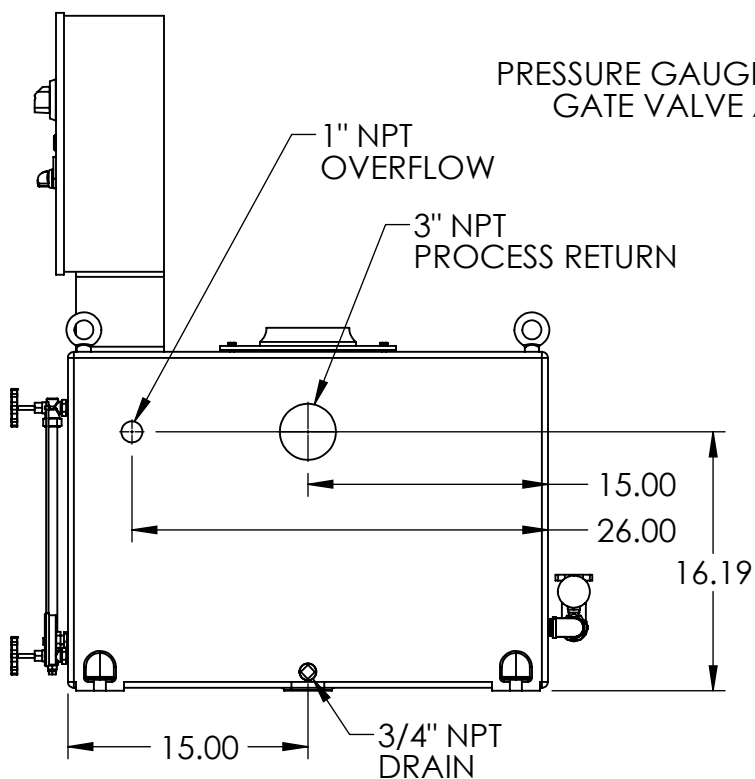
BACK VIEW
