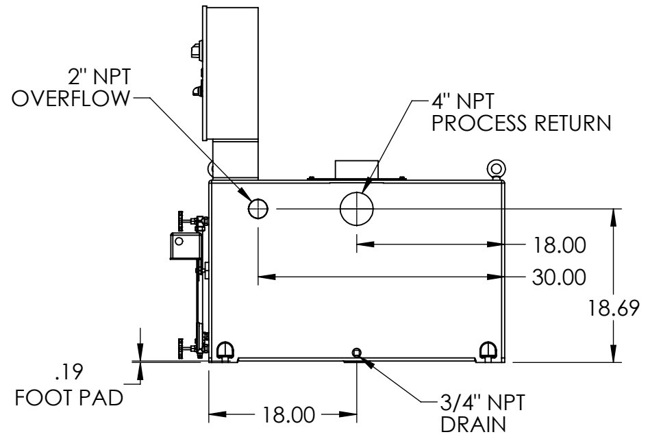
BACK VIEW
