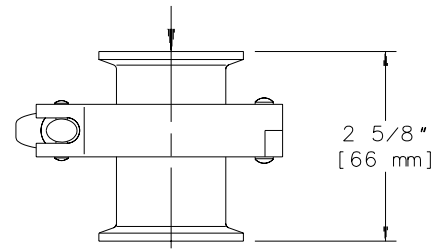
MODEL TC-C 1" SANITARY CONN.
