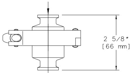
MODEL TC-C 1/2 & 3/4 SANITARY CONN.
